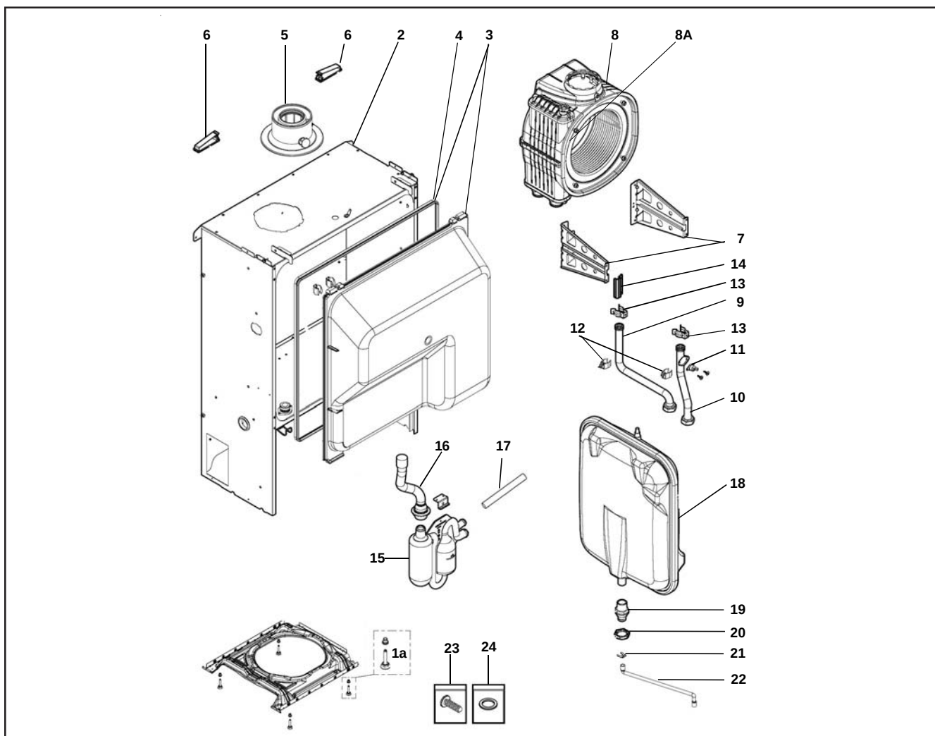
Corps - Caisson
