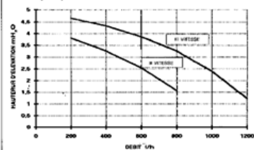
23 FF - pompe standard
