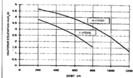
23 CF - pompe standard - 23 VMC
