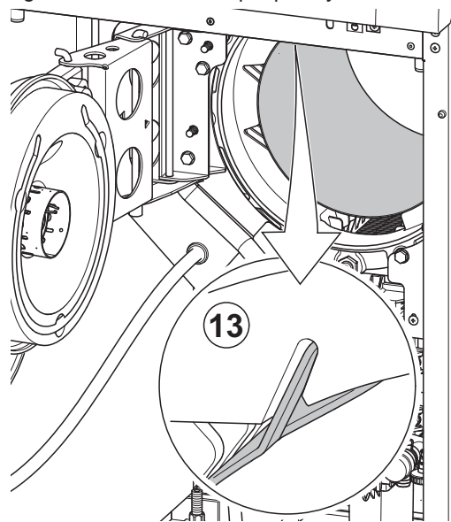
Fig.54 Insertion de la plaque foyère
