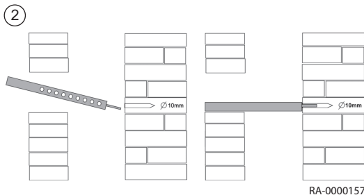
Fig.21 Montage du rail support
