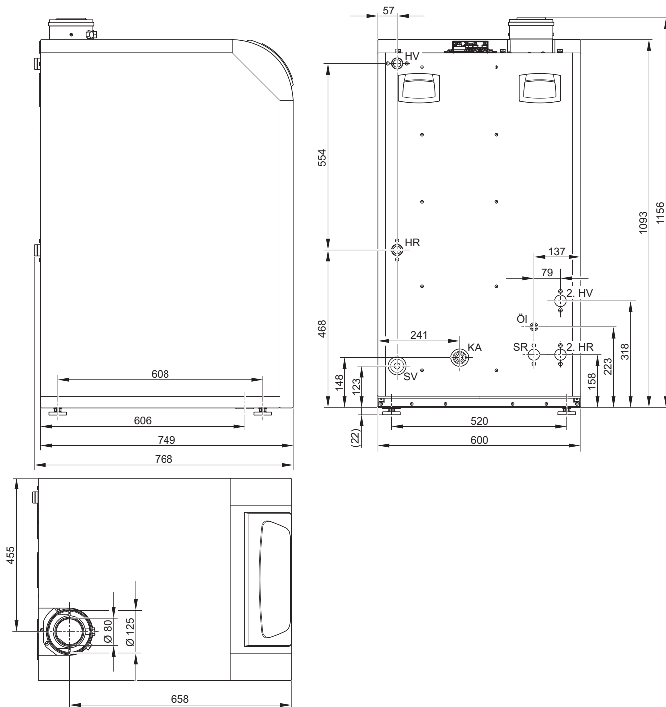
Fig.2 Dimensions et raccords BORA EVO HTE
