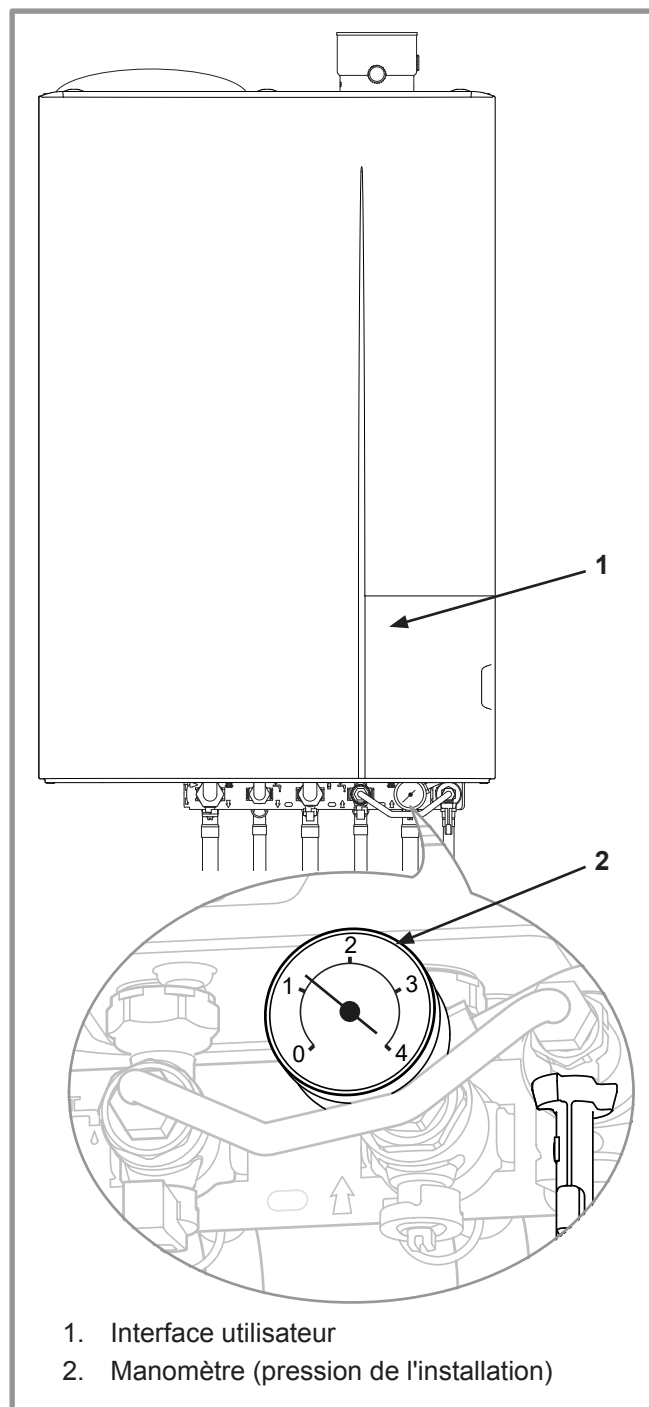
figure 1 - Chaudière Duo 35
