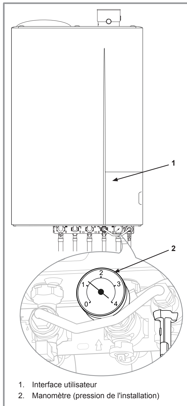
figure 1 - Chaudière Duo 35
