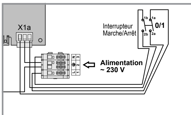
figure 26 - Raccordement alimentation
