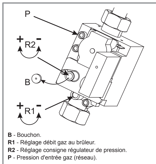
figure 32 - Vanne gaz
