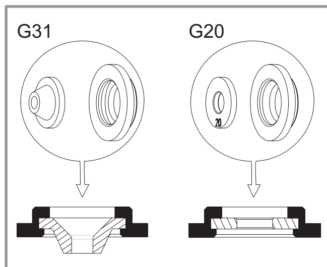
figure 19 - Diaphragme vanne gaz
