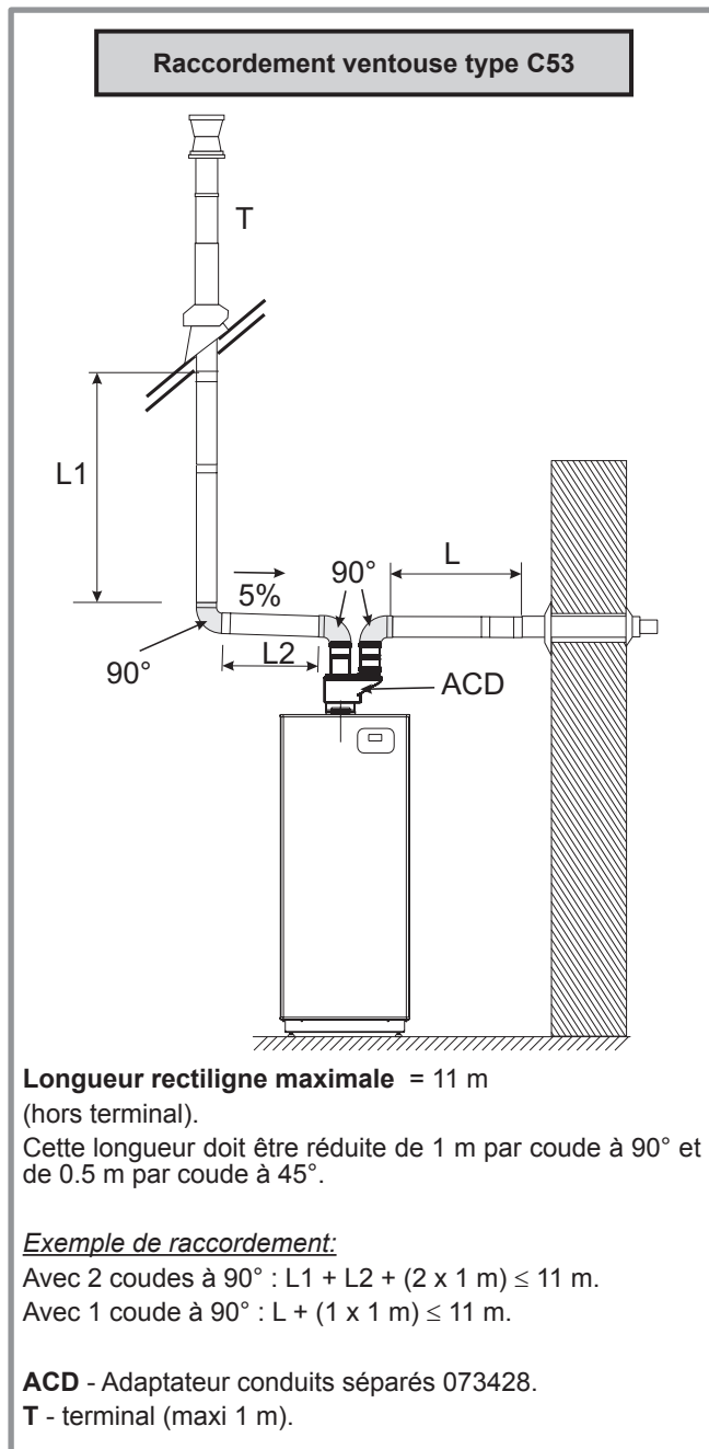
figure 22 - Possibilités de raccordement (type C53)
