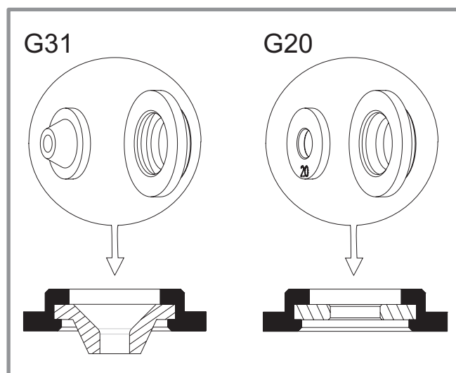
figure 35 - Diaphragme vanne gaz
