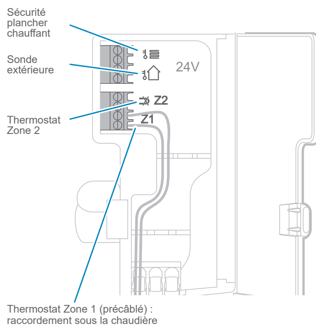
fig. 19 - Borniers TBTS
